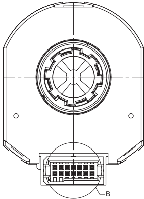
STANDARD CONNECTOR OPTION
